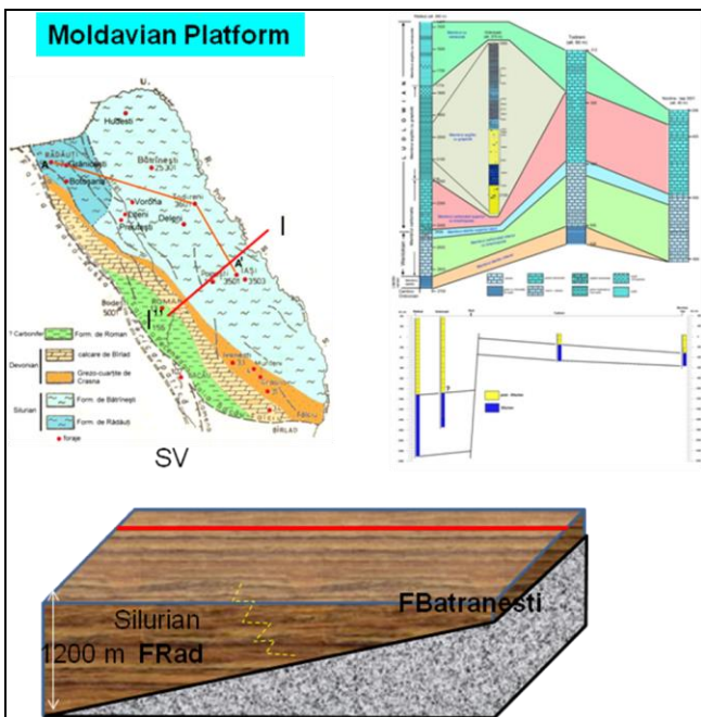
Fig. 2. Moldavian Platform – thickness of formations – Cycle I.
